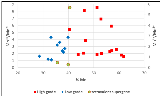
Figure 3: Plot of bulk Mn valence ratios against Mn grade of ore samples (Chetty and Gutzmer, 2018). Note, only the tetravalent supergene data points should be read against the right hand axis of Mn^{4+}/Mn^{2+} ratio.
