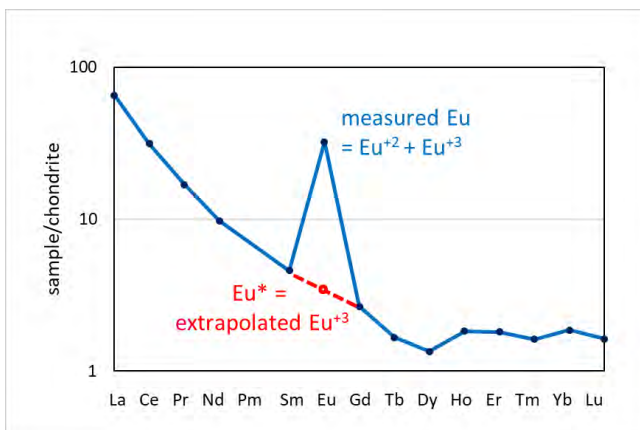
A standard chondrite-normalised REE plot, in which the valence (oxidation) state relationship between \text{Eu}^{+2} and \text{Eu}^{+3} is illustrated, for a plagioclase-rich granitoid from Namaqualand. (S. Prevec).
